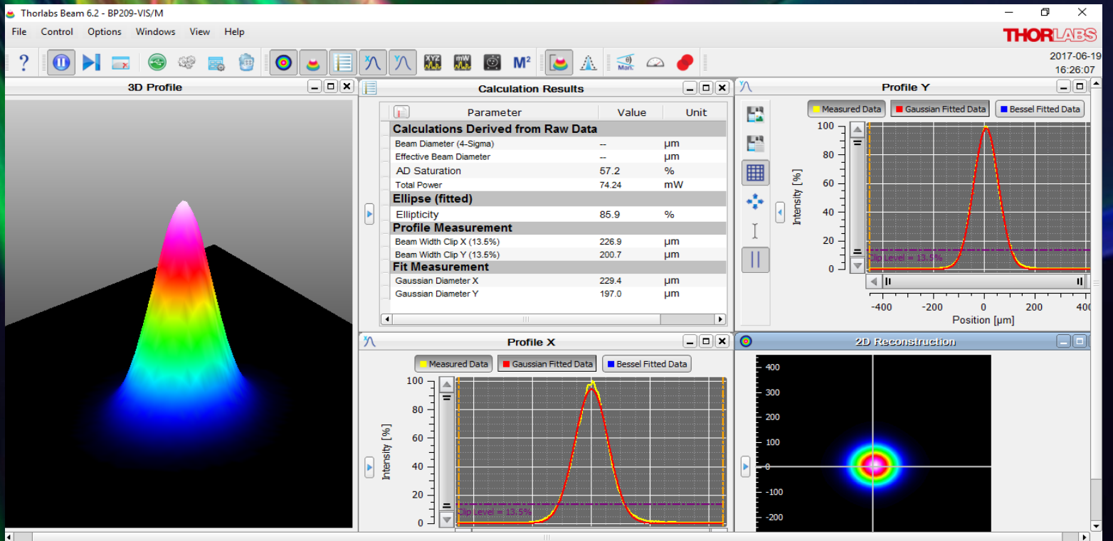
Far-field measured 60cm from laser head aperture after 50mm lens
