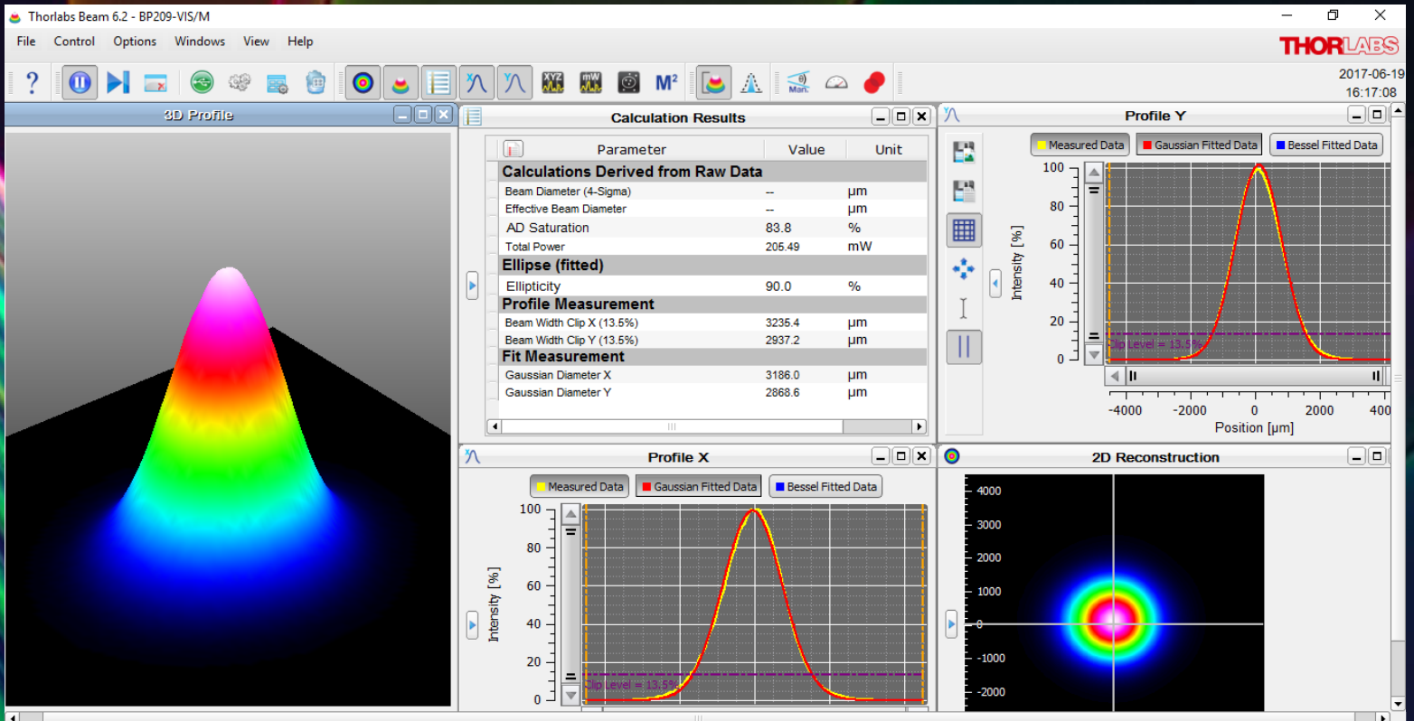
Near-field measured 60cm from laser head aperture
