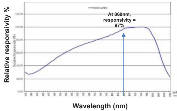
Photodiode responsivity chart
