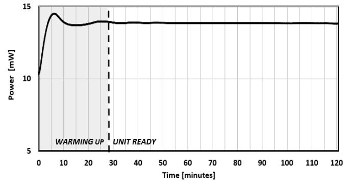
FIG. 4: WARM-UP TIME
