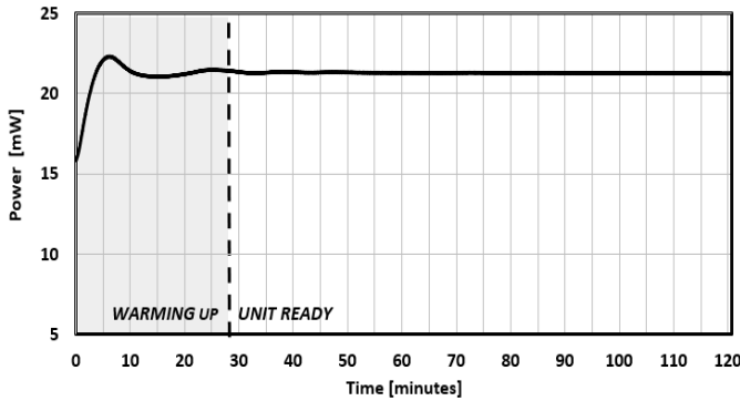
FIG. 9: WARM-UP TIME
