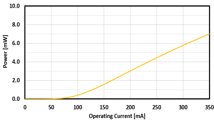
FIG. 5: SLED 2 OUTPUT POWER VS CURRENT
