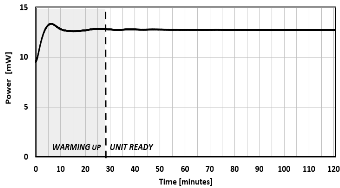
FIG. 7: WARM-UP TIME
