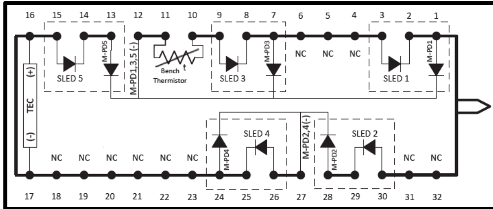
External Pin Assignment – BeST-SLED: 5 SLEDs
