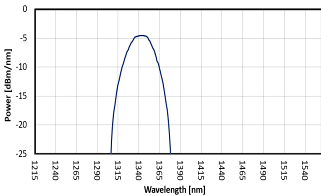
FIG. 5: SLED 4 SPECTRUM
