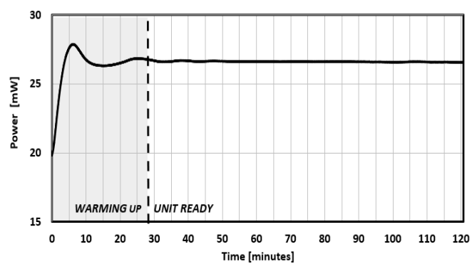
FIG. 13: WARM-UP TIME
