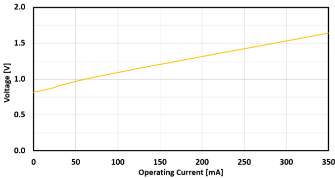
FIG. 9: SLED 2 FORWARD VOLTAGE VS CURRENT
