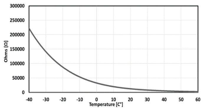
FIG. 14: THERMISTOR R_{THTEC} RESISTANCE VS TEMPERATURE
