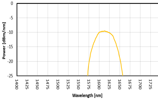
FIG. 5: SLED 4 SPECTRUM
