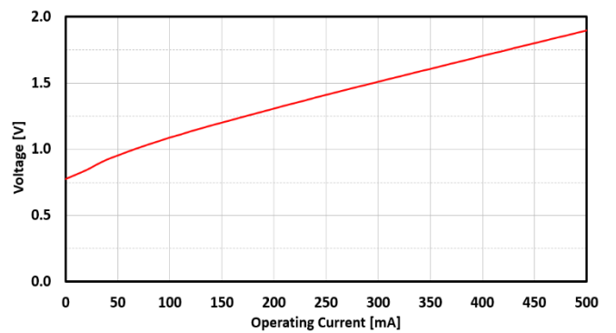
FIG. 12: SLED 3 FORWARD VOLTAGE VS CURRENT
