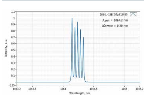
Typical spectrum of 1064 nm DPSS laser. Measured with 20 pm resolution.
