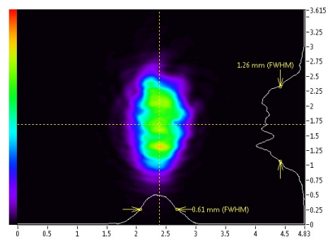
Typical near field (0.45 m from output aperture) beam profile. Non-circularized beam of a 0445 nm direct diode laser.
