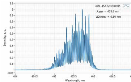
Typical spectrum of 405 nm diode laser. Measured with 10 pm resolution.
