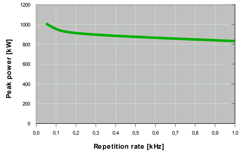
Wedge XB 1572 nm: Peak Power
