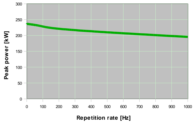
Wedge HB 355: Peak Power
