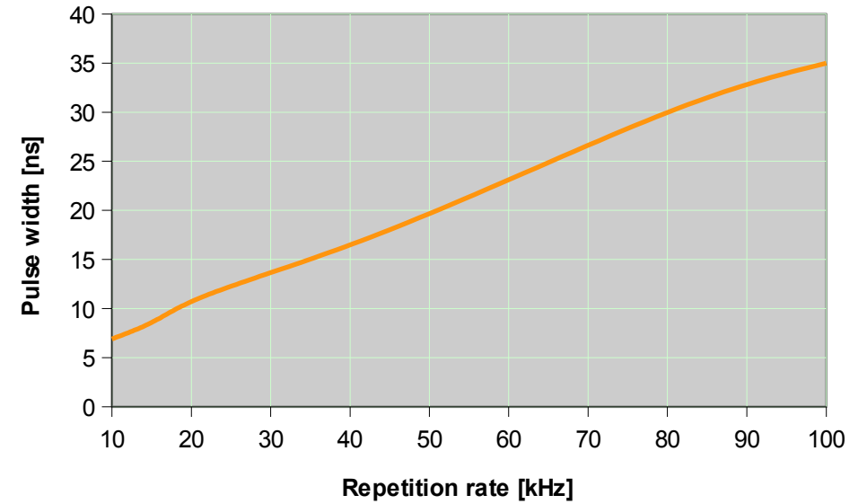
Sol 20W 1064nm: Pulse Width
