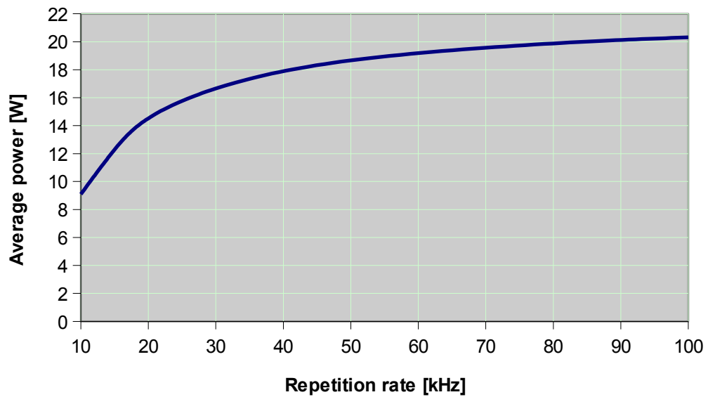
Sol 20W 1064nm: Average Power
