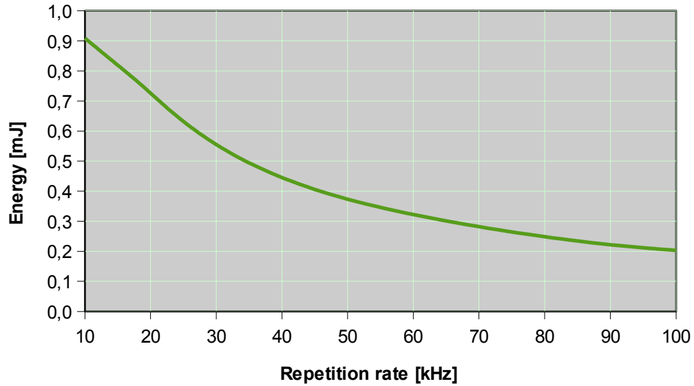
Sol 20W 1064nm: Pulse Energy
