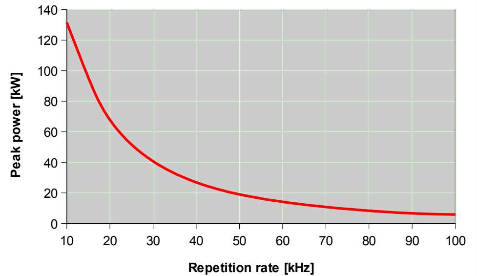
Sol 20W 1064nm: Peak Power
